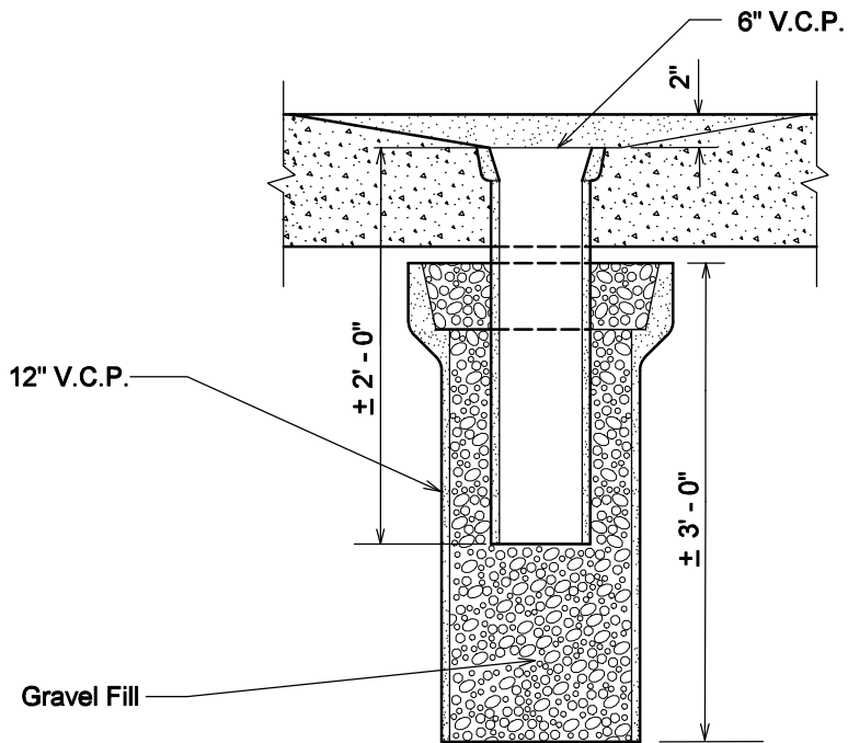
DRAIN DETAIL
