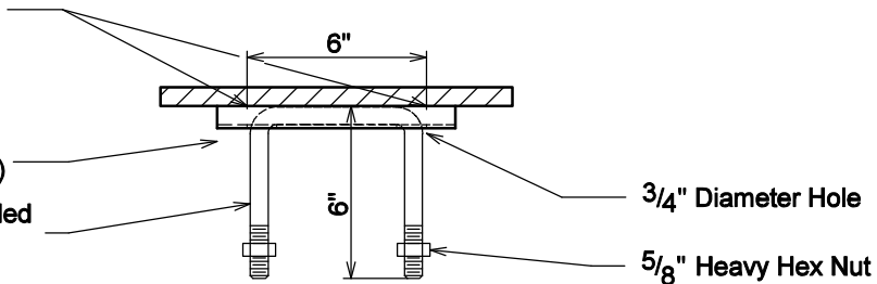
DROP HANDLE DETAIL
