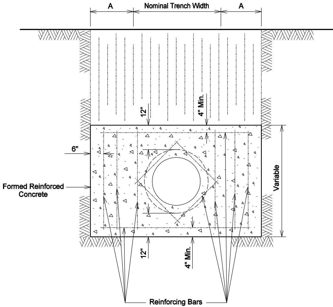
END VIEW OF REACTION BLOCK
