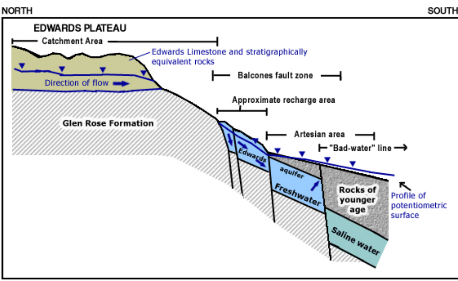
DIAGRAMMATIC CROSS SECTION
